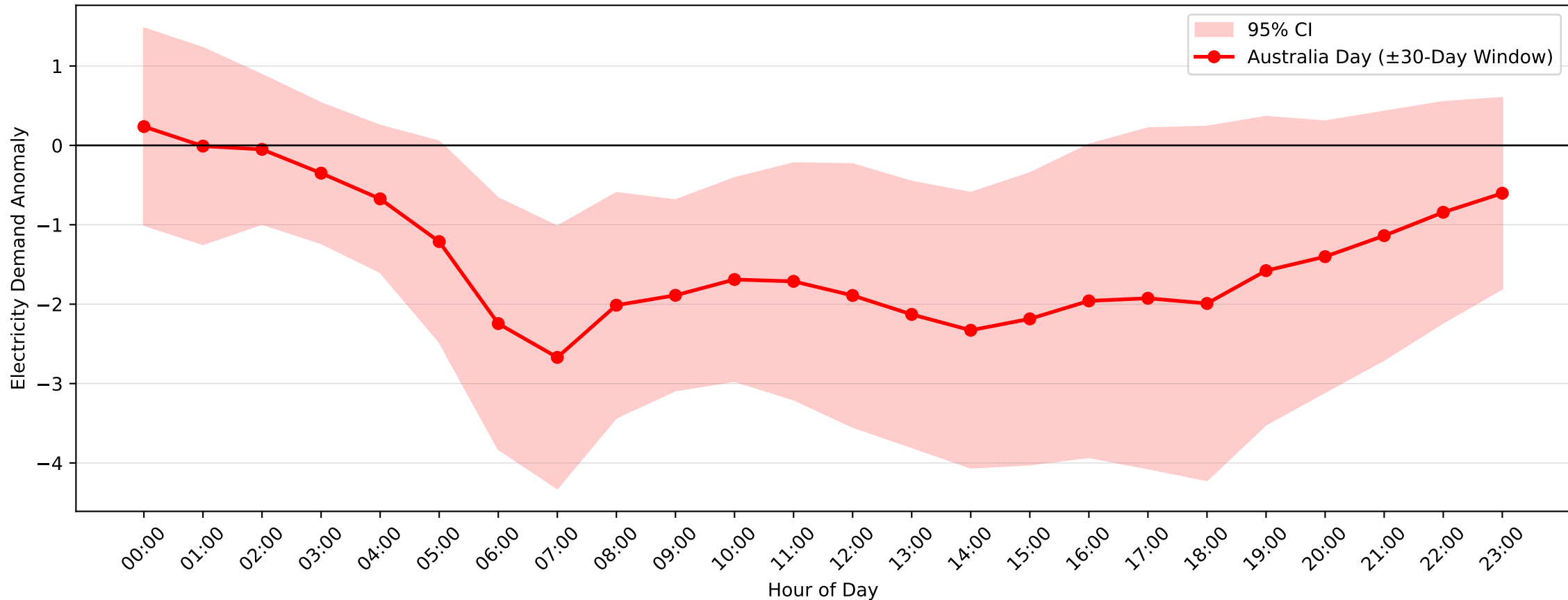
Lisarow Demand Anomaly: Australia Day (2004-2017, \pm 30 -Day Window)
